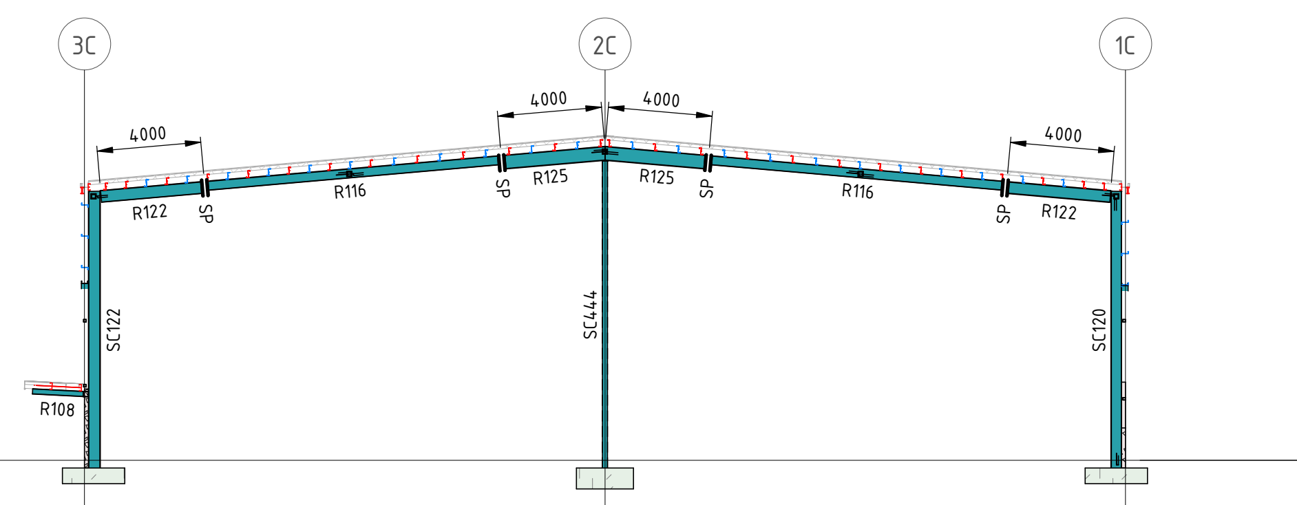
SECTION C9 SCALE 1 : 200 006502
