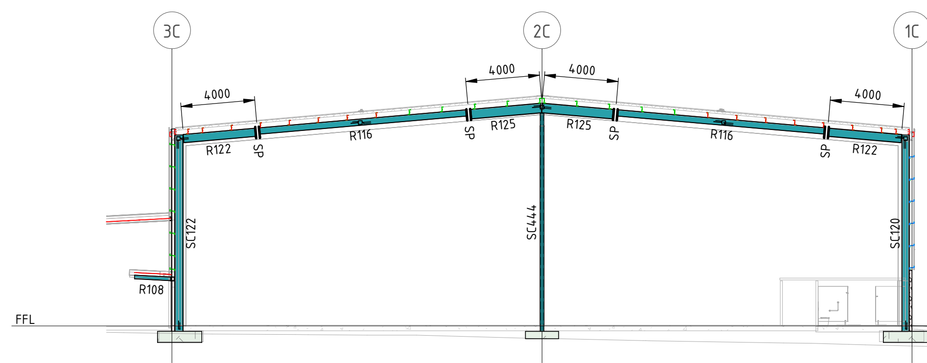
SECTION C2 SCALE 1 : 200 006002
