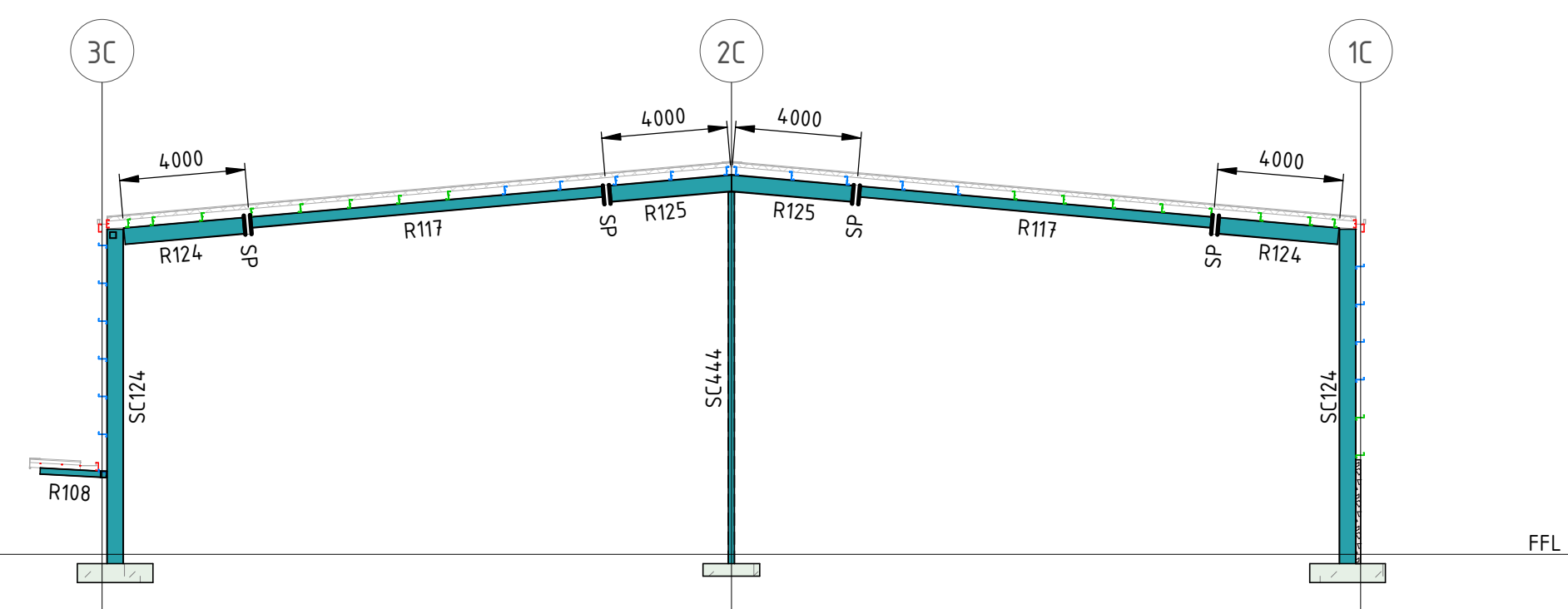
SECTION C7 SCALE 1 : 200 006502
