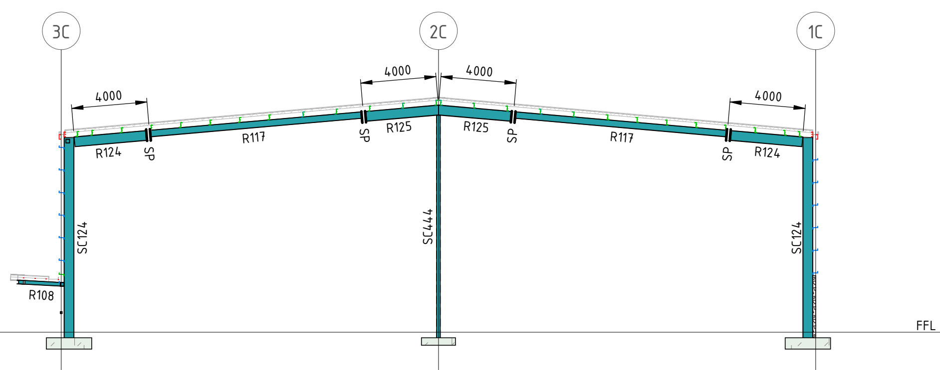
SECTION C3 SCALE 1 : 200 002002
