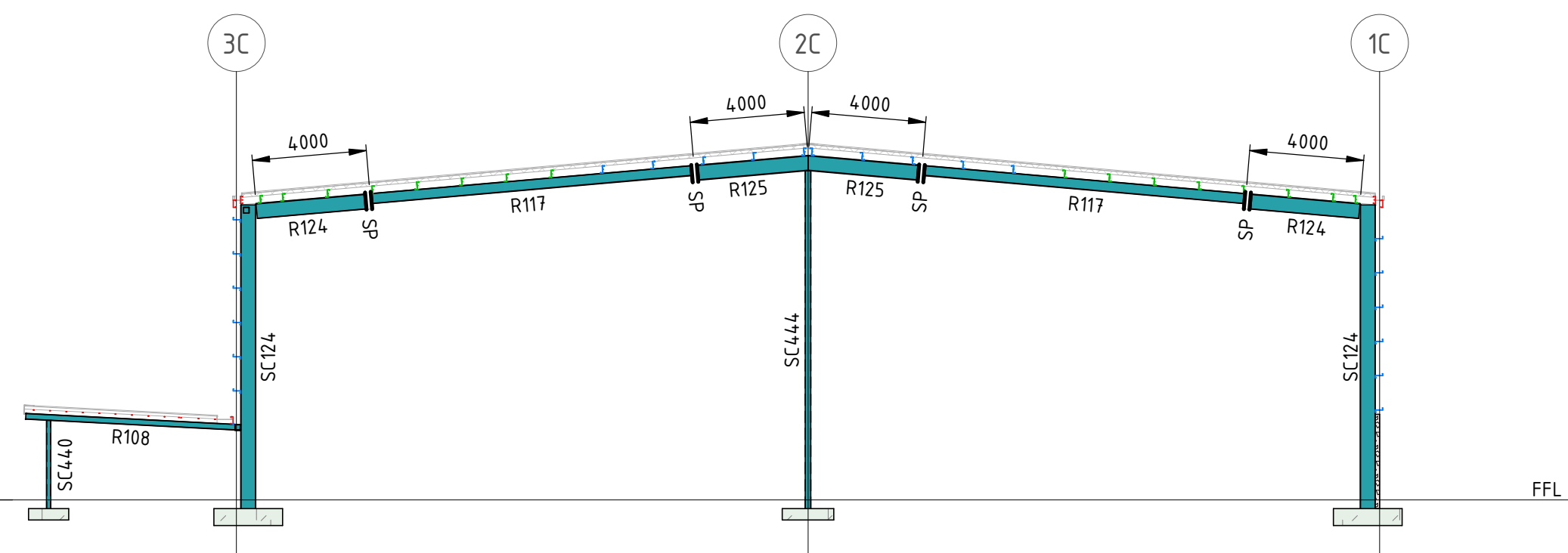
SECTION C5 SCALE 1 : 200 006502
